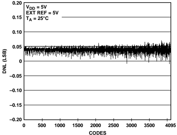
Figure 8. DNL AD5629R—External Reference
