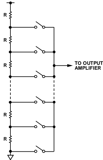
Figure 49. Resistor String
