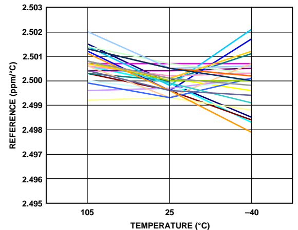
Figure 46. 2.5 V Reference Temperature Coefficient vs. Temperature
