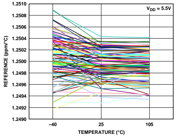
Figure 45. 1.25 V Reference Temperature Coefficient vs. Temperature
