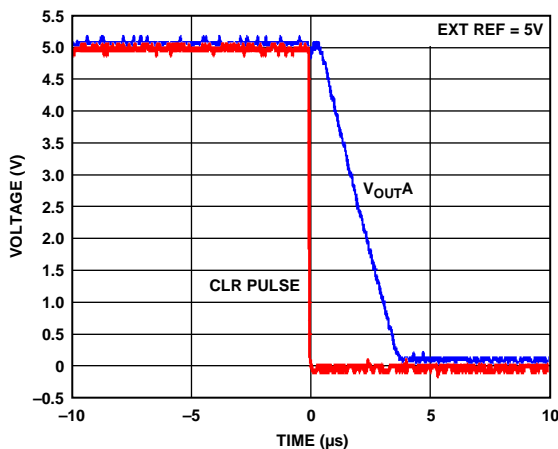
Figure 43. Hardware CLR
