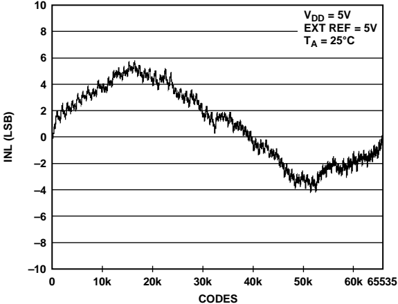
Figure 5. INL AD5669R—External Reference
