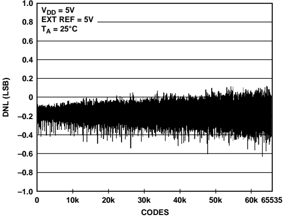
Figure 7. DNL AD5669R—External Reference
