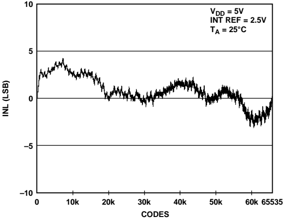
Figure 9. INL AD5669R-2—Internal Reference
