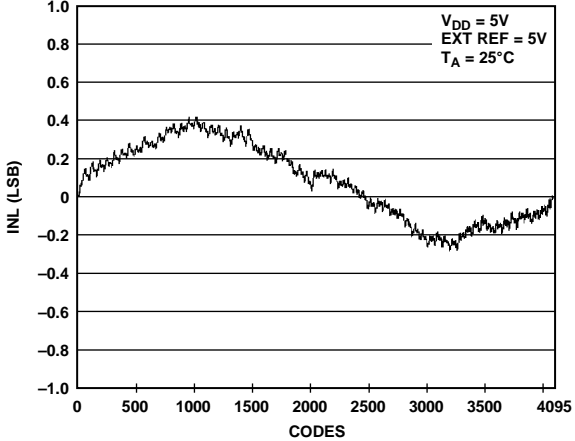
Figure 6. INL AD5629R—External Reference
