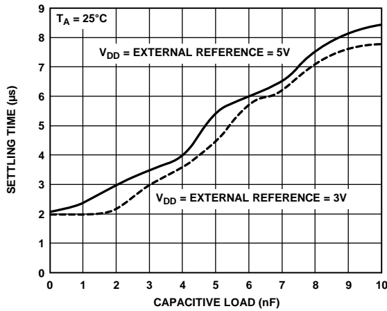
Figure 42. Settling Time vs. Capacitive Load
