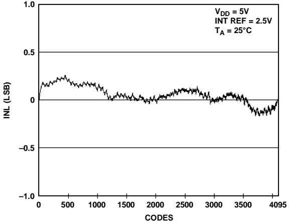
Figure 10. INL AD5629R-2—Internal Reference
